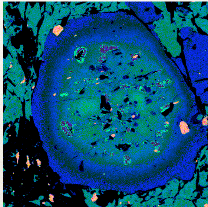
Image of CaK \alpha in garnet from the Blue Ridge, North Carolina
