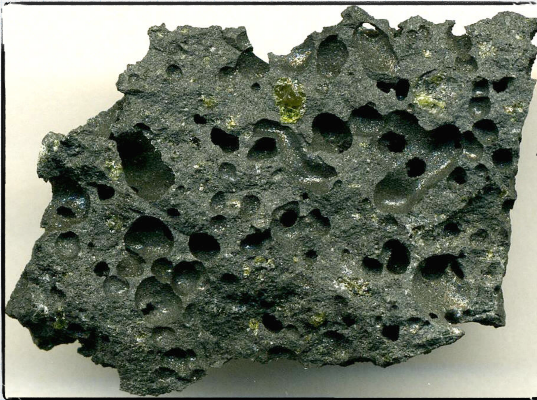
Mt. Kilauea volcanic lava - February 1960 vesicular porphyritic olivine basalt, erupted from the East Rift Zone of Kilauea Volcano, Hawaii Hotspot.
