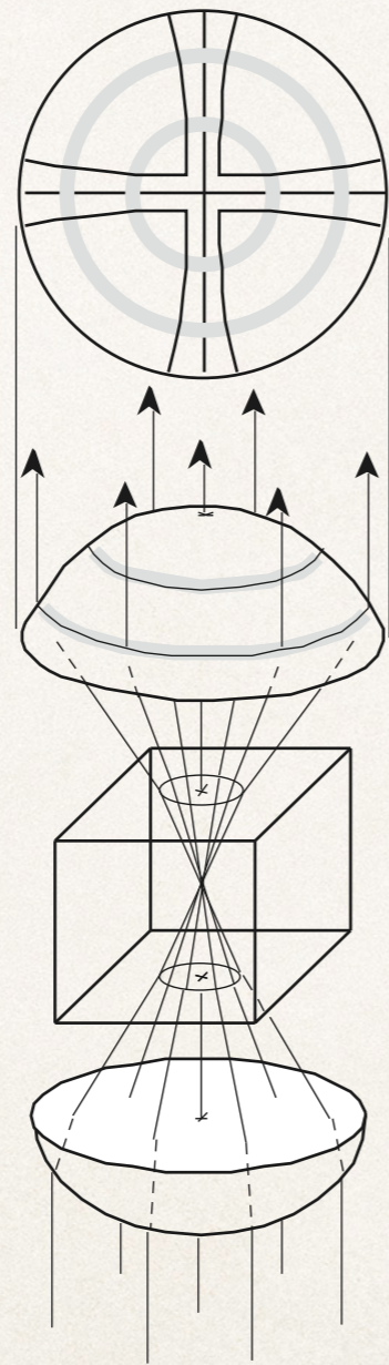
Retardation in convergent polarized light (conoscopic view). from Nesse
