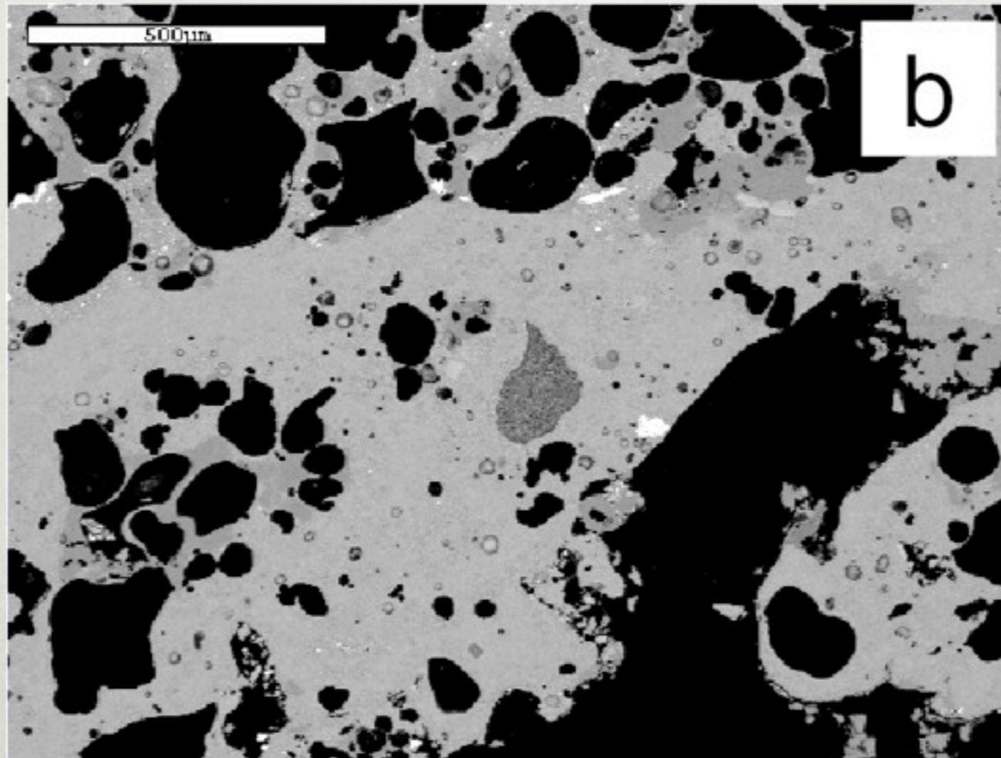
(b) basaltic impact melt
