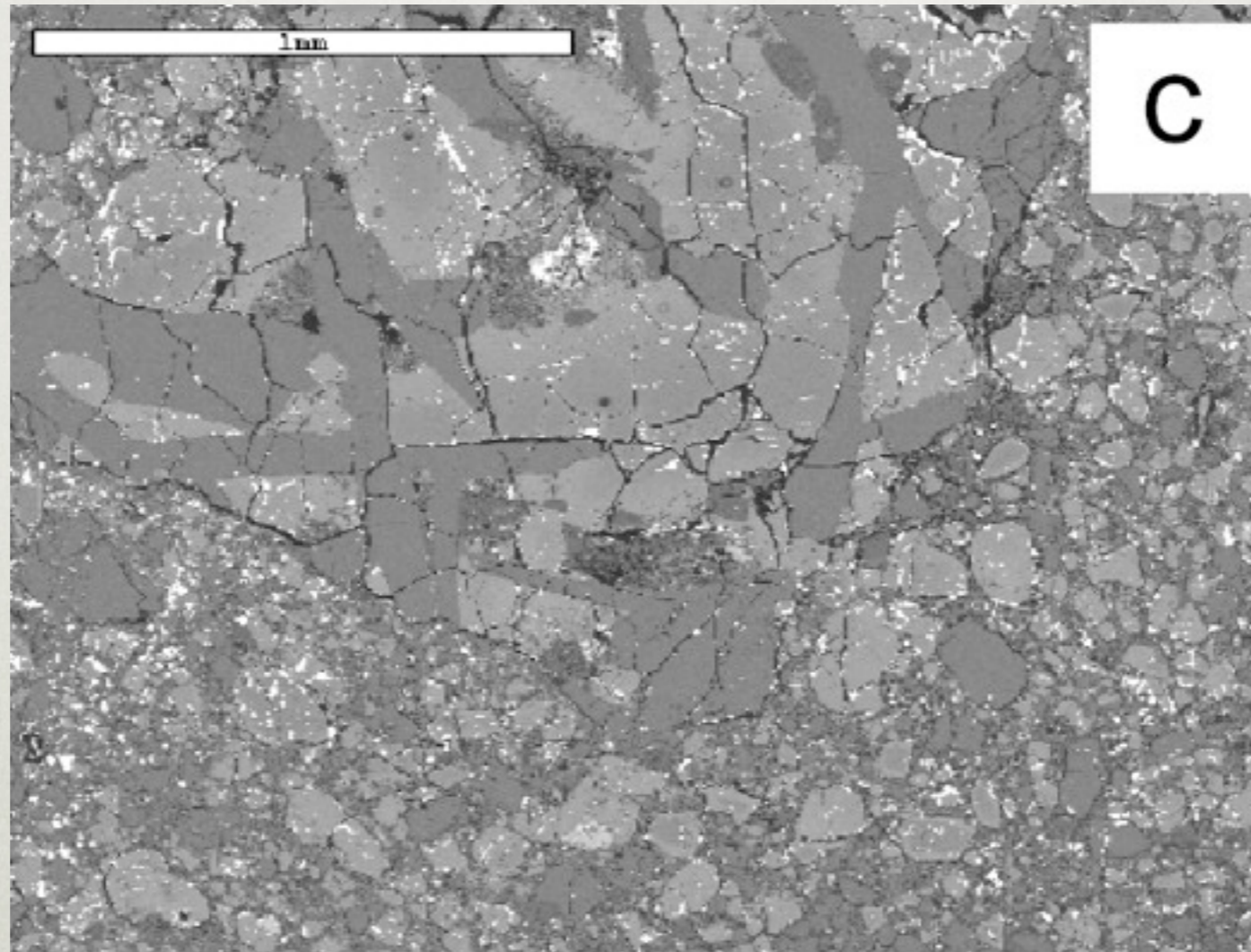
(c) basaltic breccia
