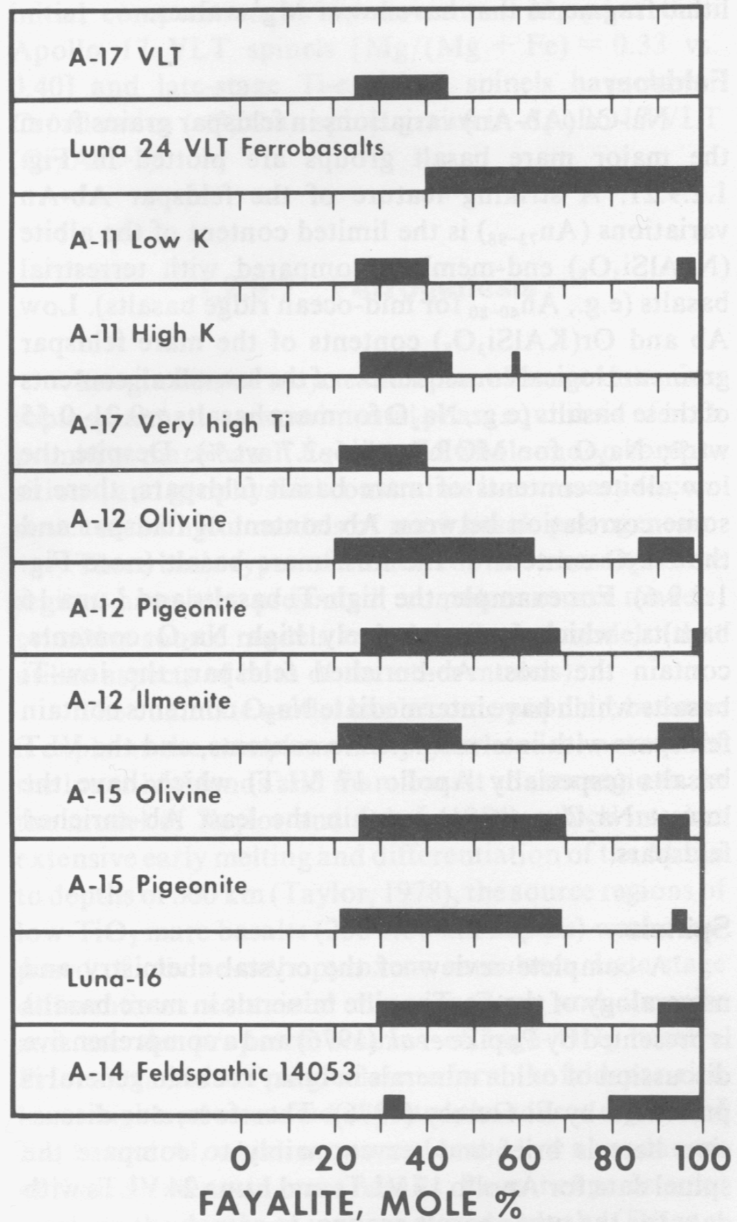
1.2.9.20 Fayalite contents of mare basalt olivines.
