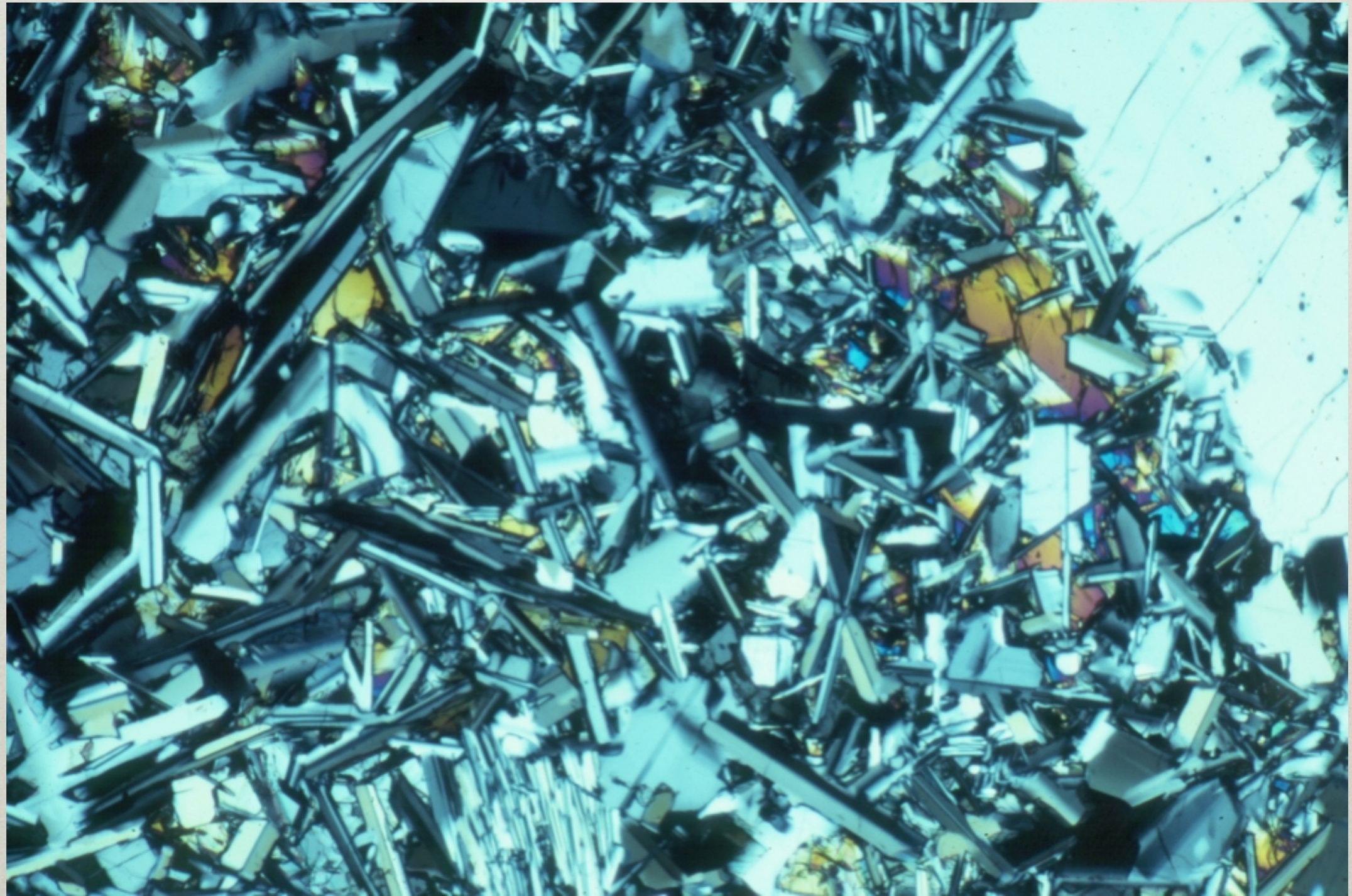
Highlands Anorthosite 65055
