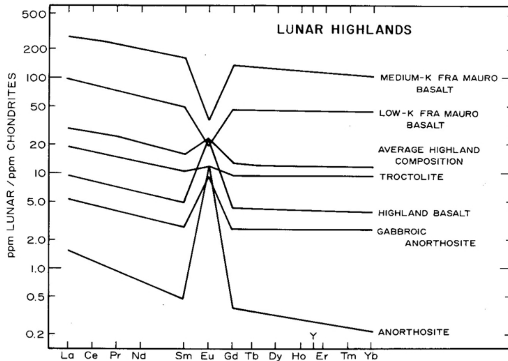
Fig. 5.20 Rare earth element (REE) abundances in highland rock types [89, 92]. Note that the average highland composition has a positive Eu anomaly. The slopes of the patterns are nearly parallel. The La/Yb ratio is close to 3.1 for most patterns, except for the plagioclase-rich samples, where the La/Yb ratio rises.
