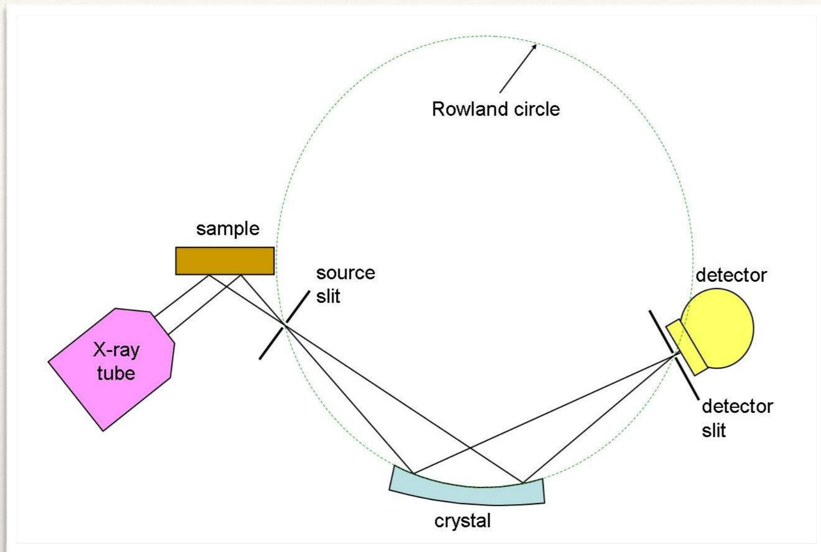
Wavelength-dispersive XRF
