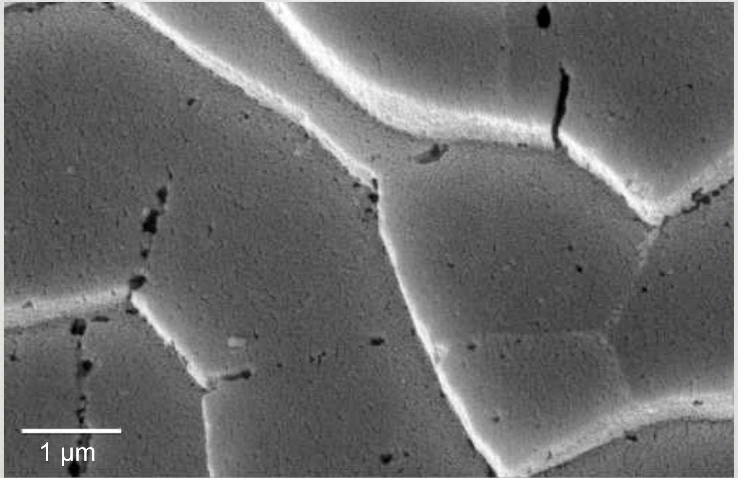
Figure 14. SEM micrograph of red abalone nacre tiles seen at a fractured edge.
