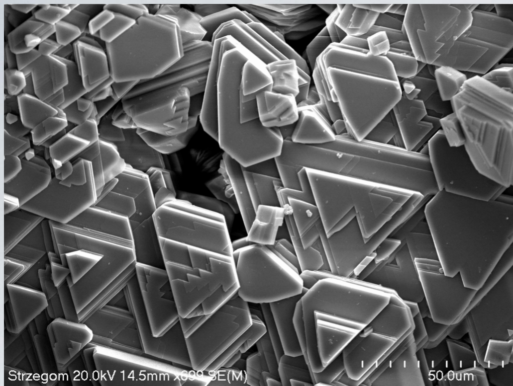
Fe and Al rich chlorite from Strzegom pegmatite (Poland). Local name for this mineral is strzegomite
