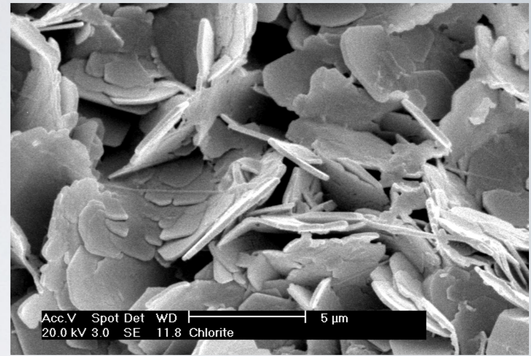
Mg-rich chlorite, Rotliegend, Northern Germany
