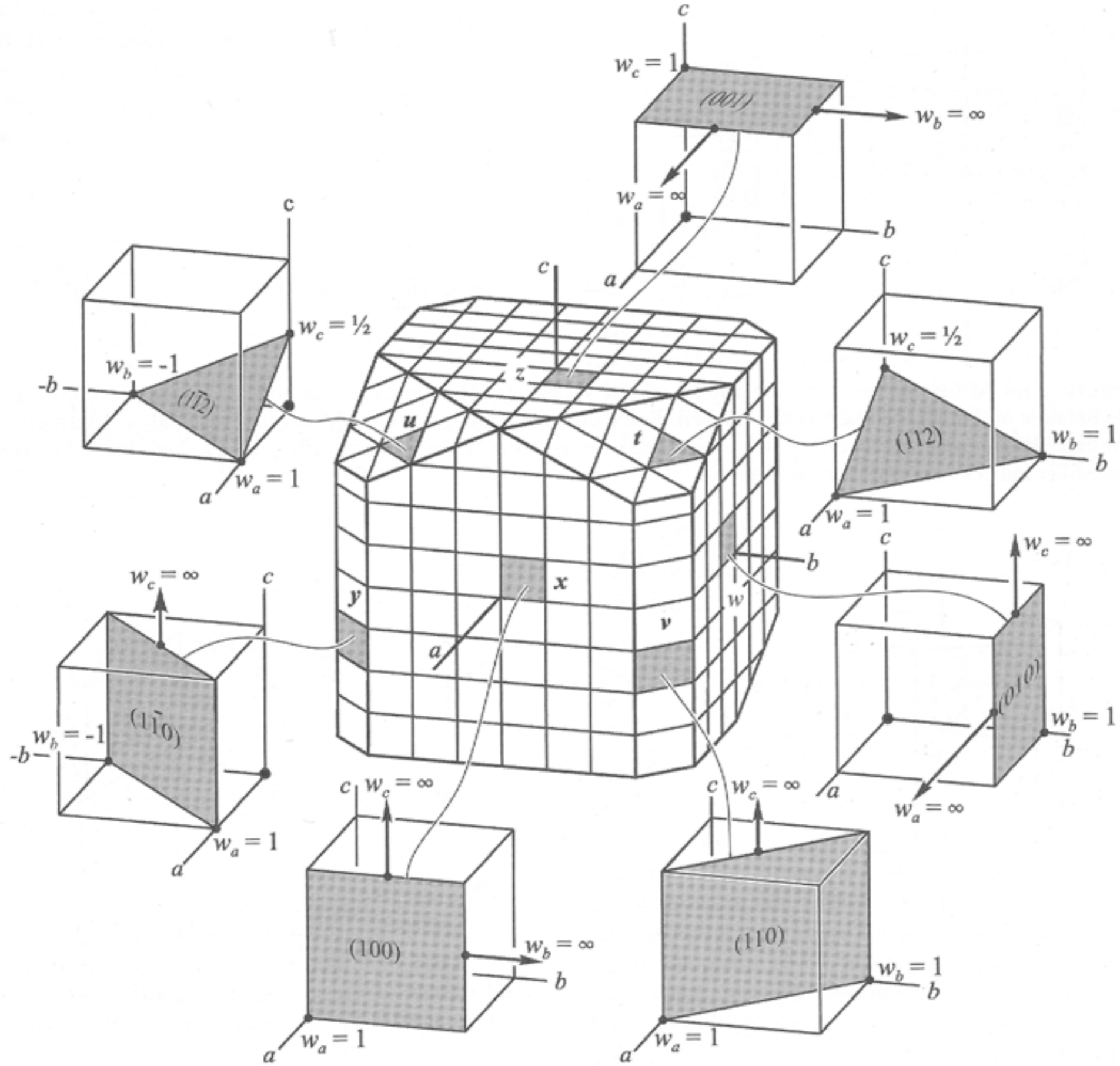
Figure 2.23 Miller indices for all visible faces on the crystal shown in Figure 2.22. The traces of unit cells are sketched on the crystal. See text for discussion.
