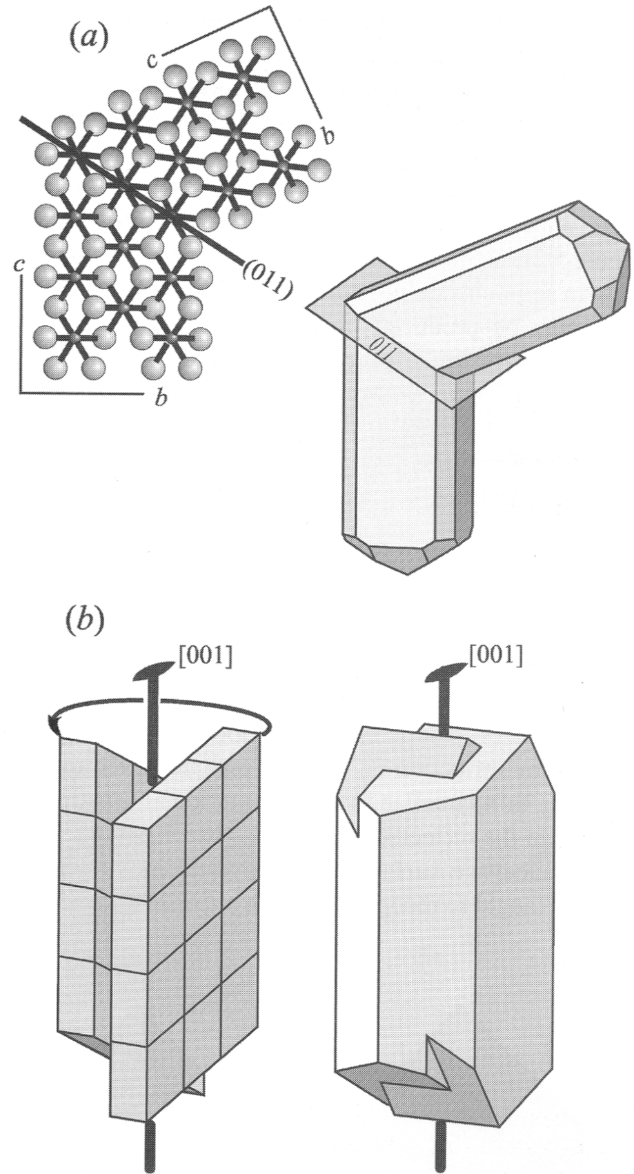
Figure 5.20 Symmetry operations in twinning. (a) Twinning by reflection on {011} in rutile. (b) Twinning by rotation on [001] in K-feldspar to produce a Carlsbad twin.
