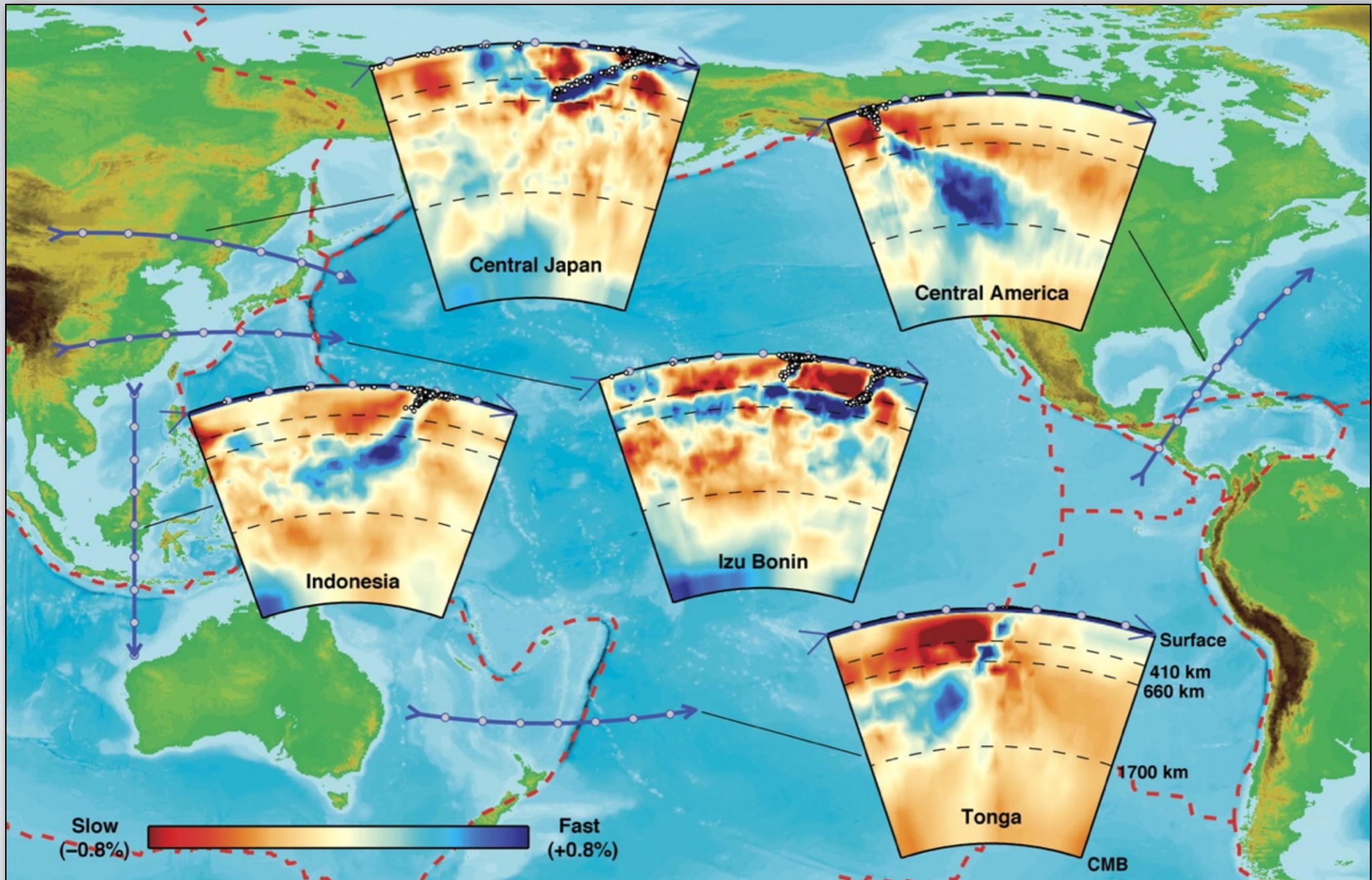
3-D tomographic structure of the mantle near several subduction zones in the western Pacific and central America. Note the differences in structure and apparent trajectories of subducted slabs in different subduction zones.
