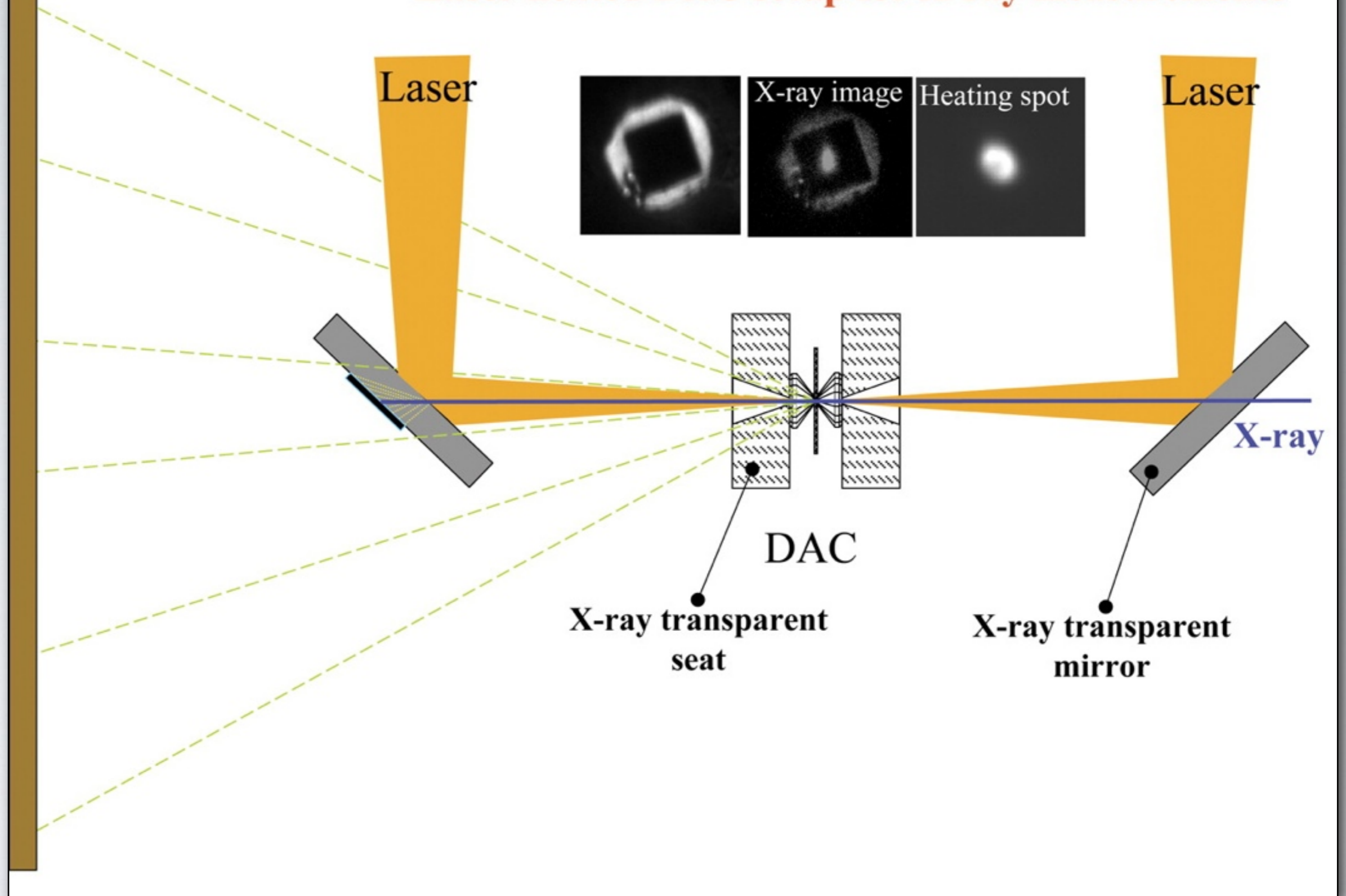
Schematic diagram of a diamond anvil cell (DAC), with the sample heated from both sides with lasers. The inset photographs show the sample in the sample chamber of the DAC, with laser heating at right.
