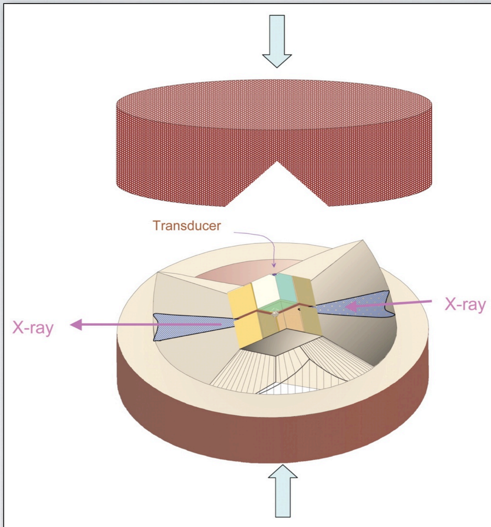
Schematic diagram of a two-stage Kawai-type multi-anvil apparatus. The eight inner cubes are anvils that compress an octahedron-shaped sample assembly. The transducer produces an ultrasonic signal that is transmitted to the sample and detects the return signal.
