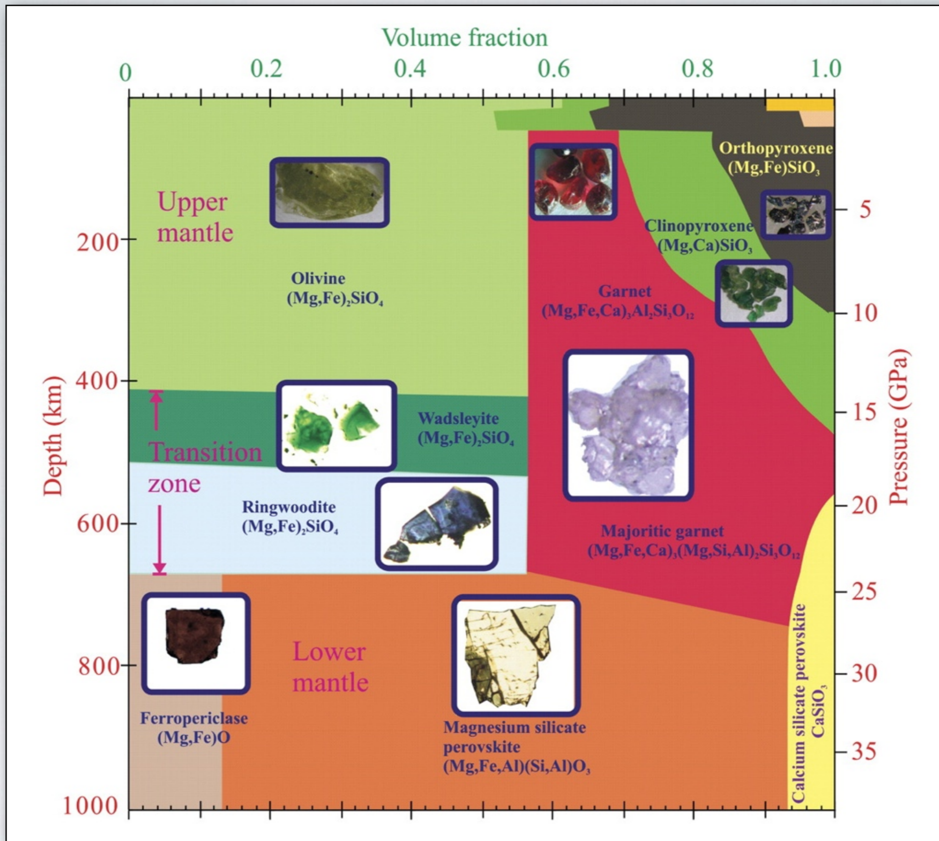
Mineral volume fractions for the top 1000 km of a pyrolite mantle. Small orange and pink regions in the top-right-hand corner denote the stabilities of feldspar and spinel, respectively.
