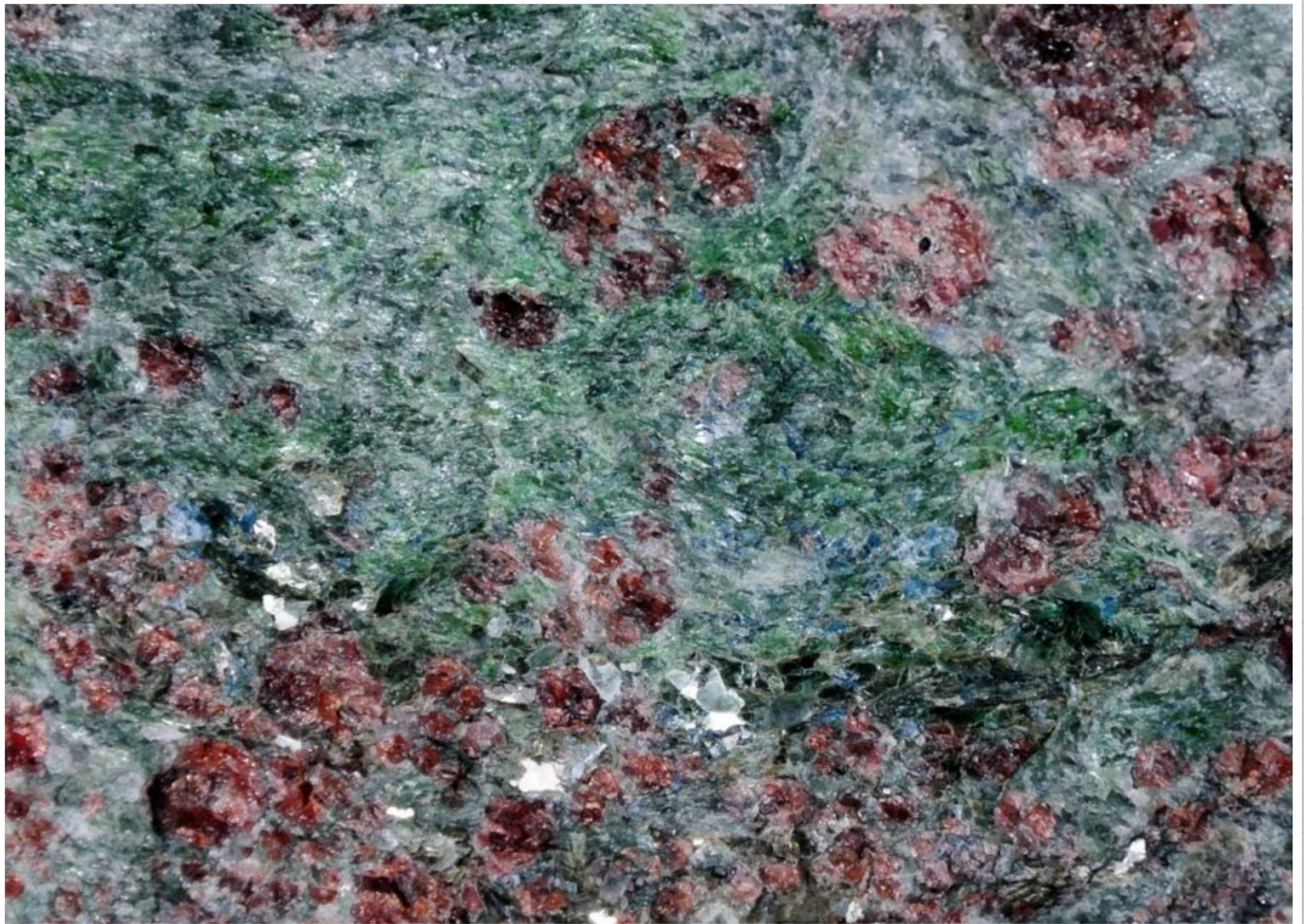
Eclogite, Nordfjord. Red-brown garnet, green omphacite, bluish kyanite.
