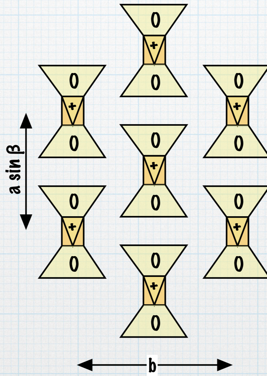
C2/c Diopside structure
