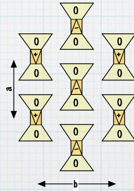
Pbcn Protopyroxene structure
