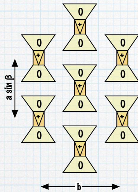
C2/c Diopside structure
