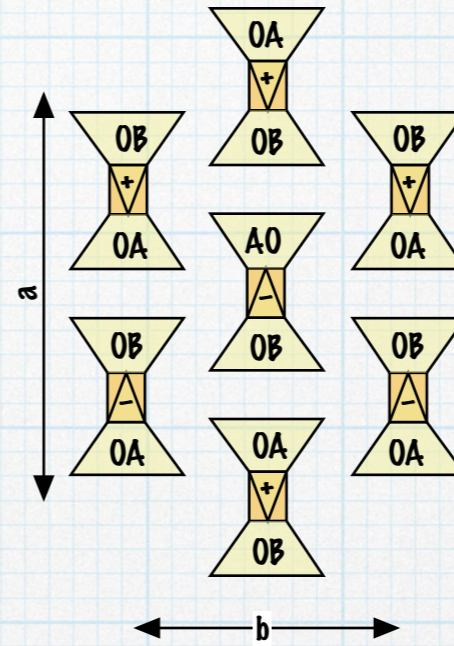
Pbc Orthopyroxene structure
