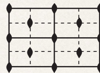
c2mm
