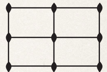
p2mm
