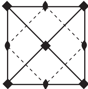
p4mm
