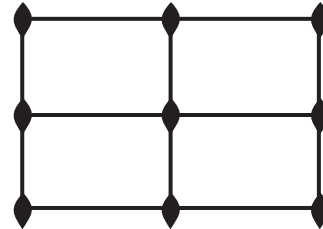
p2mm
