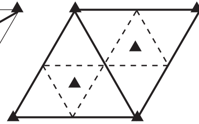
p31m
