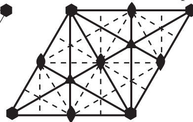
p6mm
