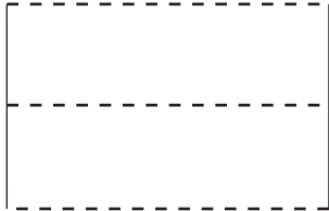
pg
